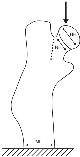
Fig. 1. Mouse proximal femur in anterior view. With the distal femur fixed, load is applied to the femoral head to cause cantilever bending at the femoral neck. The arrow indicates the point of load application. The most common fracture orientation is marked with a dashed line. A subset of the morphometric traits which were measured are shown, including mediolateral femoral diameter (ML), femoral head height (HH), and height of the femoral neck (NH). Anteroposterior diameter, femoral head depth, and depth of the femoral neck were measured perpendicular to ML, HH, and NH, respectively.
