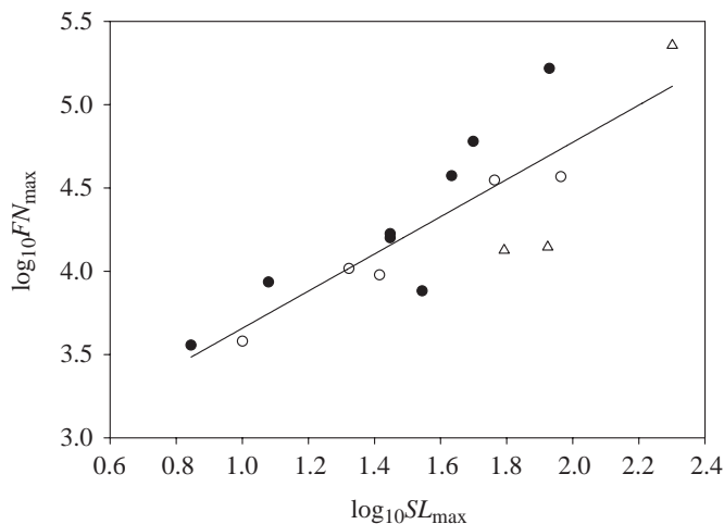
Fig. 7. The relationship between \log_{10} maximum fibre number ( FN_{max} ; data from Fig. 8) and \log_{10} maximum standard length ( SL_{max} ; data from Table 1) among 16 species of notothenioid fishes from Tierra del Fuego (filled circles), Shag Rocks, South Georgia (open triangles) and the Antarctic Peninsula (open circles). A conventional least-squares linear regression was fitted to the data. The equation was: \log_{10} FN_{max} = 2.53 + \log_{10} SL_{max} \times 1.12 ( F_{1,14} = 30.8 , P < 0.0001 ; r^2 = 0.69 ).
