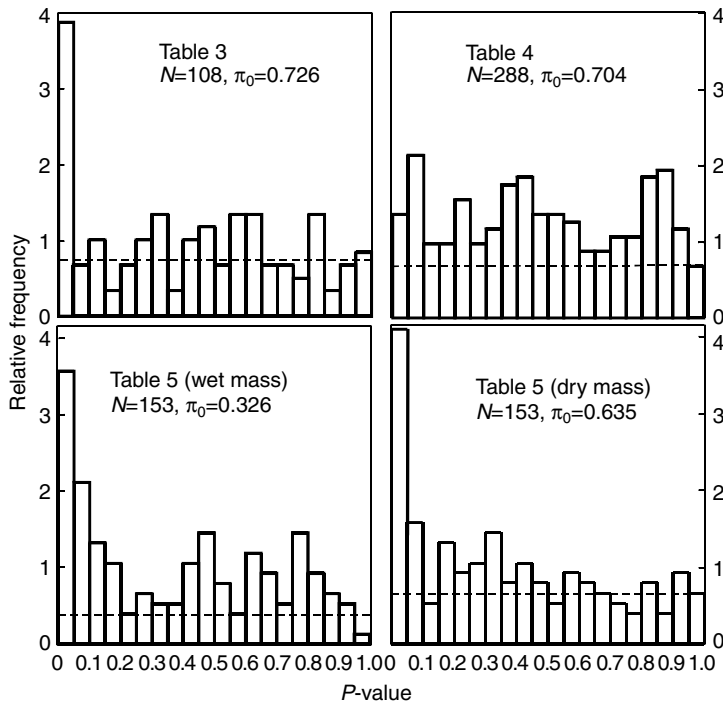
Fig. 5. Distributions of P values in relation to the \pi_0 statistic [the overall proportion of true null hypotheses (Storey and Tibshirani, 2003; Storey, 2003)] for the correlations in Tables 3–5. The bin size is 0.05; \pi_0 is shown as broken lines. A random set of P -values would produce a flat histogram with all bins showing a relative frequency close to 1.0; the presence of non-null hypotheses (i.e. significant tests after accounting for Type 1 errors) is indicated by high relative frequencies in the left-most bin. Values of \pi_0 were computed with the R program ‘Qvalue’.
